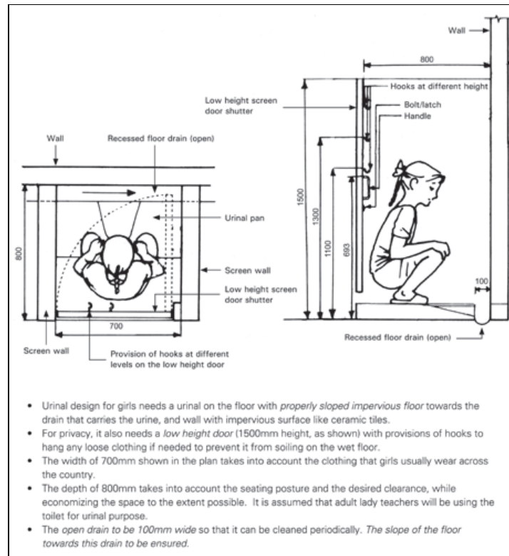
Figure 1: Girls Urinal Specifications
